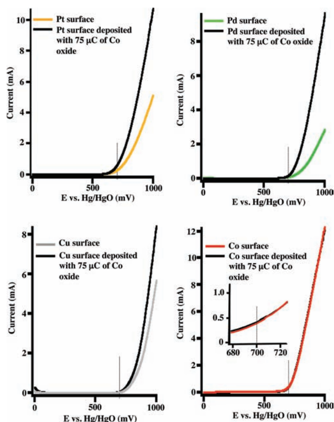
Figure 4. Linear sweep voltammograms of various metal electrodes in 0.1 M KOH. The scans are taken at 1 mV/s. A blow-up of the LSV curves of Co is included. The dotted line marks 700 mV.
